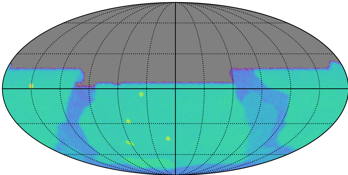
weather_cloudso35v3.5_10yrs u: SurfaceBrightLimit
