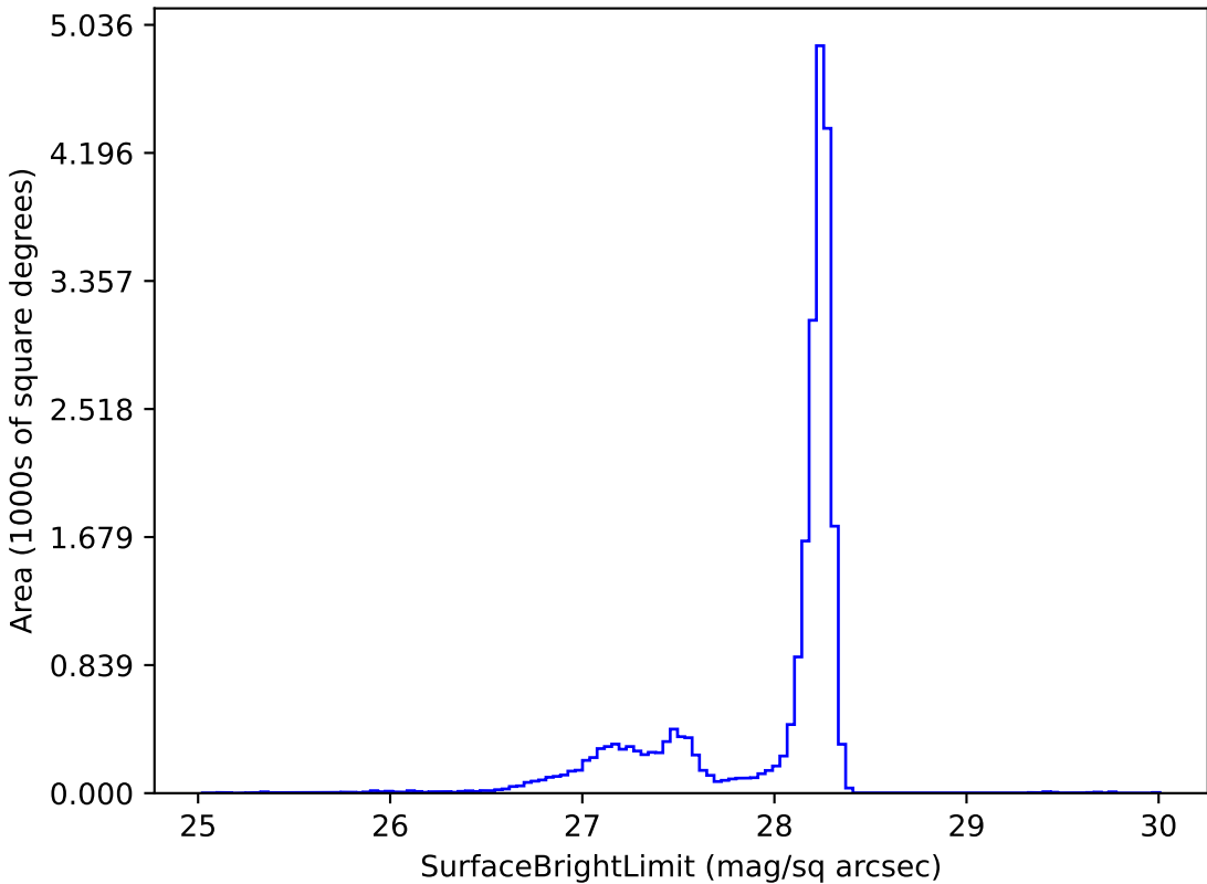
weather_cloudso35v3.5_10yrs y: SurfaceBrightLimit
