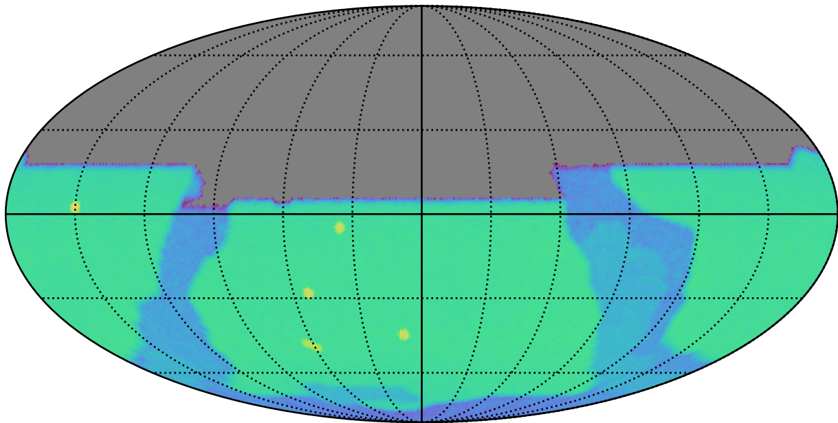
weather_cloudso35v3.5_10yrs y: SurfaceBrightLimit
