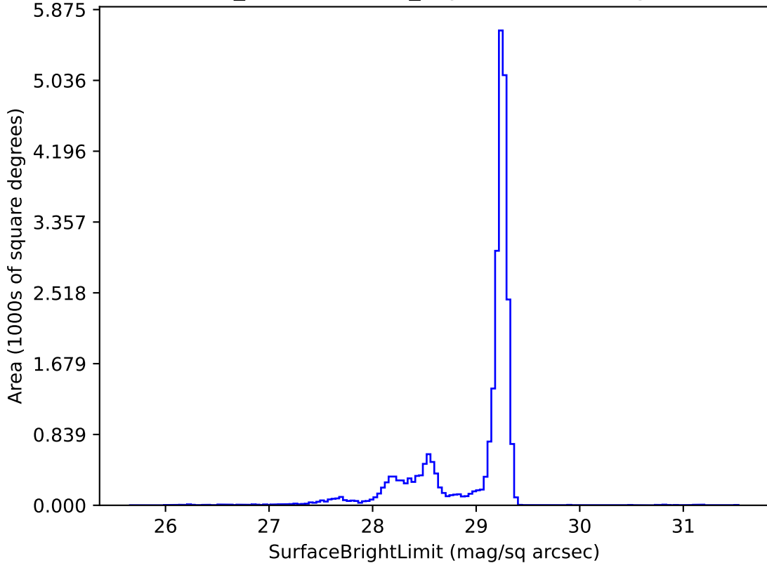
weather_cloudso35v3.5_10yrs z: SurfaceBrightLimit
