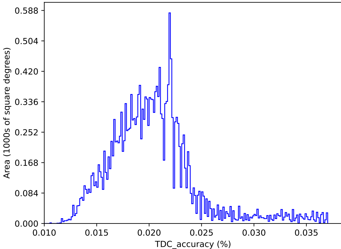
weather_cloudso35v3.5_10yrs : TDC_accuracy
