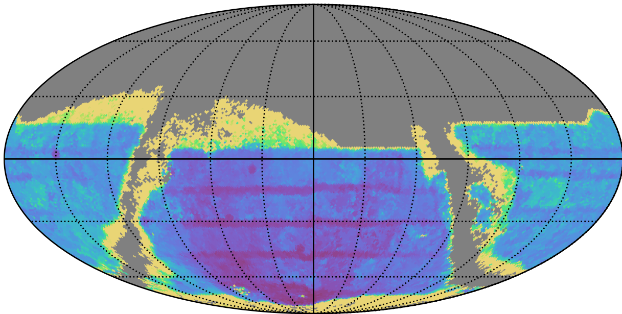
weather_cloudso35v3.5_10yrs : TDC_accuracy
