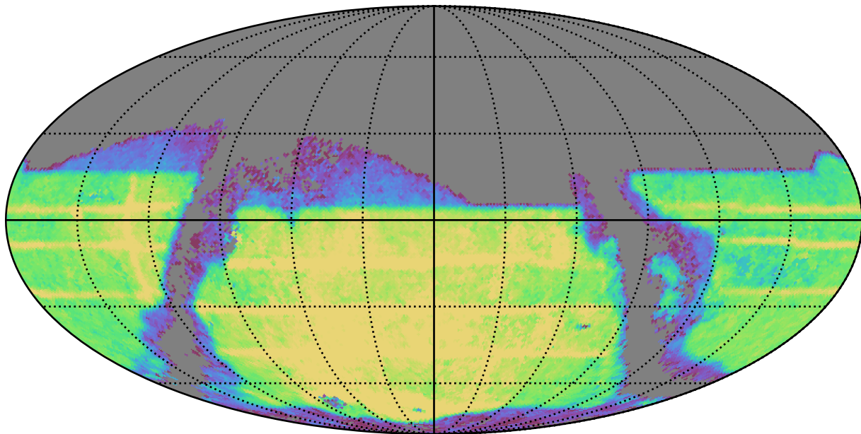
weather_cloudso35v3.5_10yrs : TDC_rate
