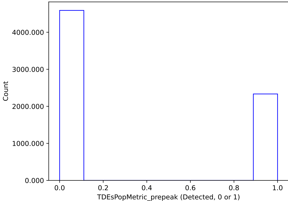
weather_cloudso35v3.5_10yrs : TDEsPopMetric_prepeak
