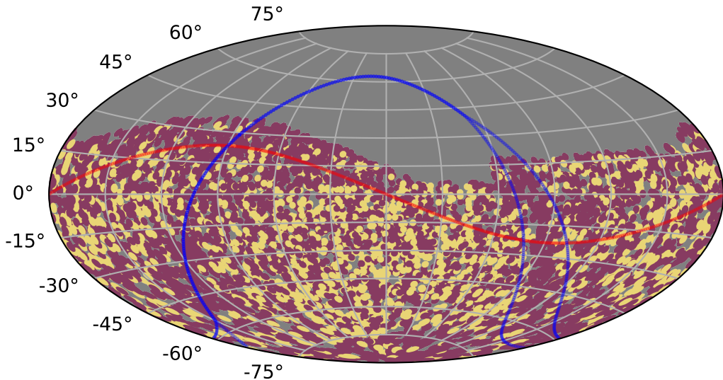
weather_cloudso35v3.5_10yrs : TDEsPopMetric_prepeak
