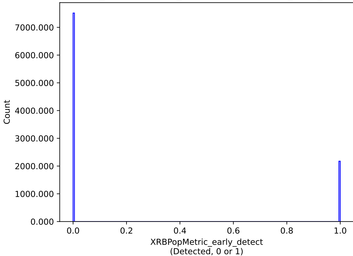
weather_cloudso35v3.5_10yrs : XRBPoMetric_early_detect
