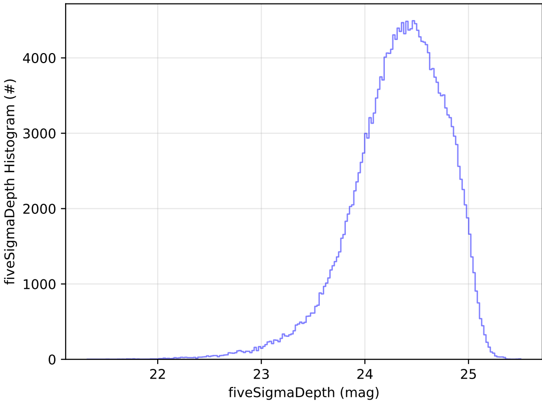
weather_cloudso35v3.5_10yrs g: fiveSigmaDepth Histogram
