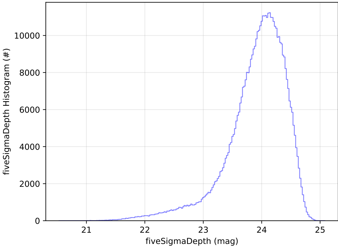
weather_cloudso35v3.5_10yrs r: fiveSigmaDepth Histogram
