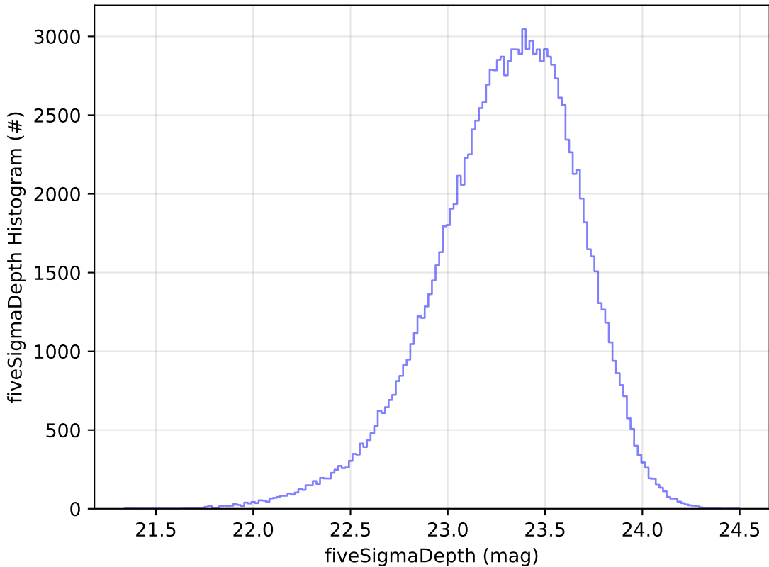
weather_cloudso35v3.5_10yrs u: fiveSigmaDepth Histogram
