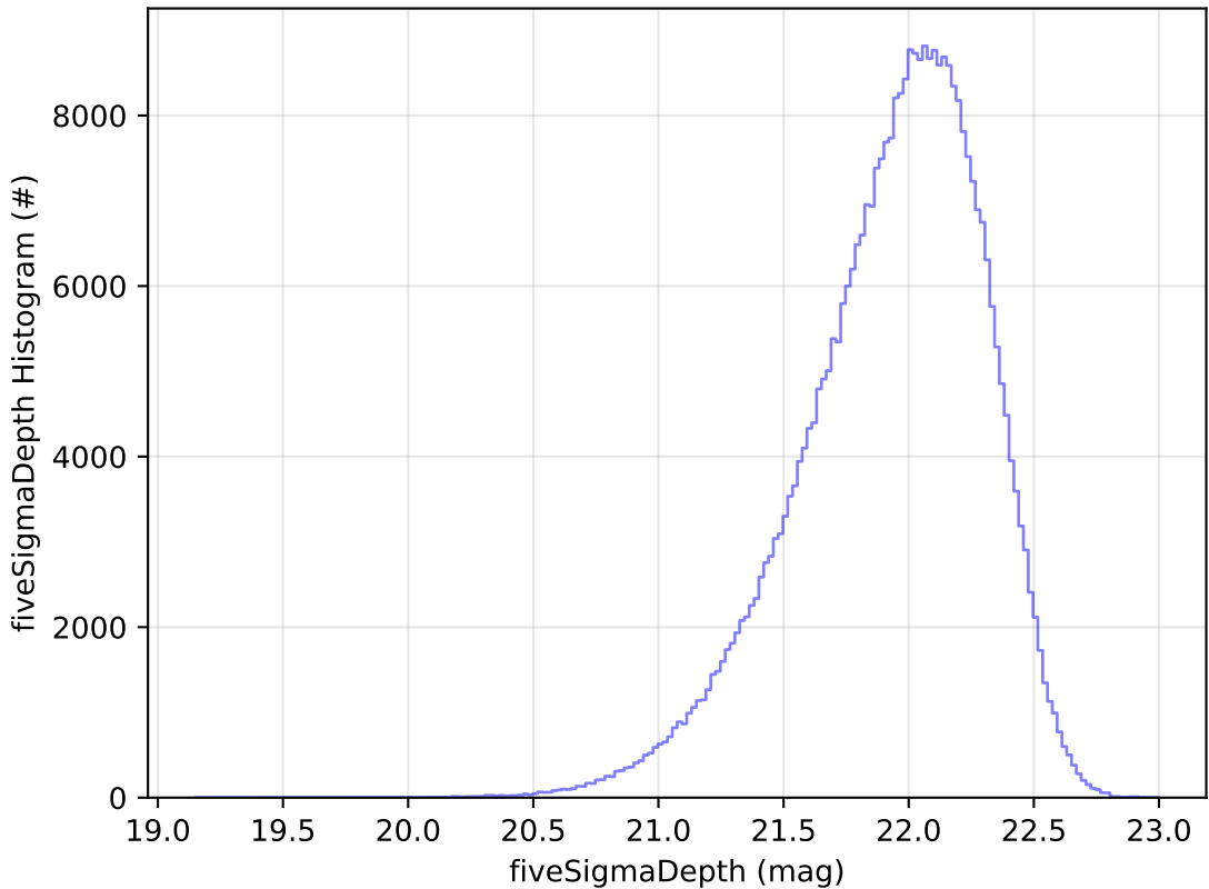
weather_cloudso35v3.5_10yrs y: fiveSigmaDepth Histogram
