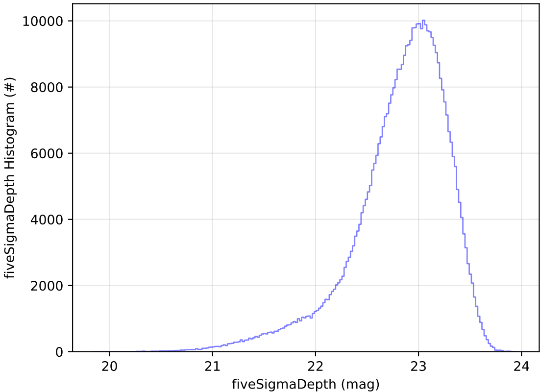
weather_cloudso35v3.5_10yrs z: fiveSigmaDepth Histogram
