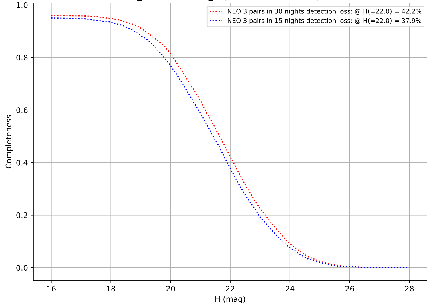
weather_cloudso35v3.5_10yrs: DifferentialCompleteness
