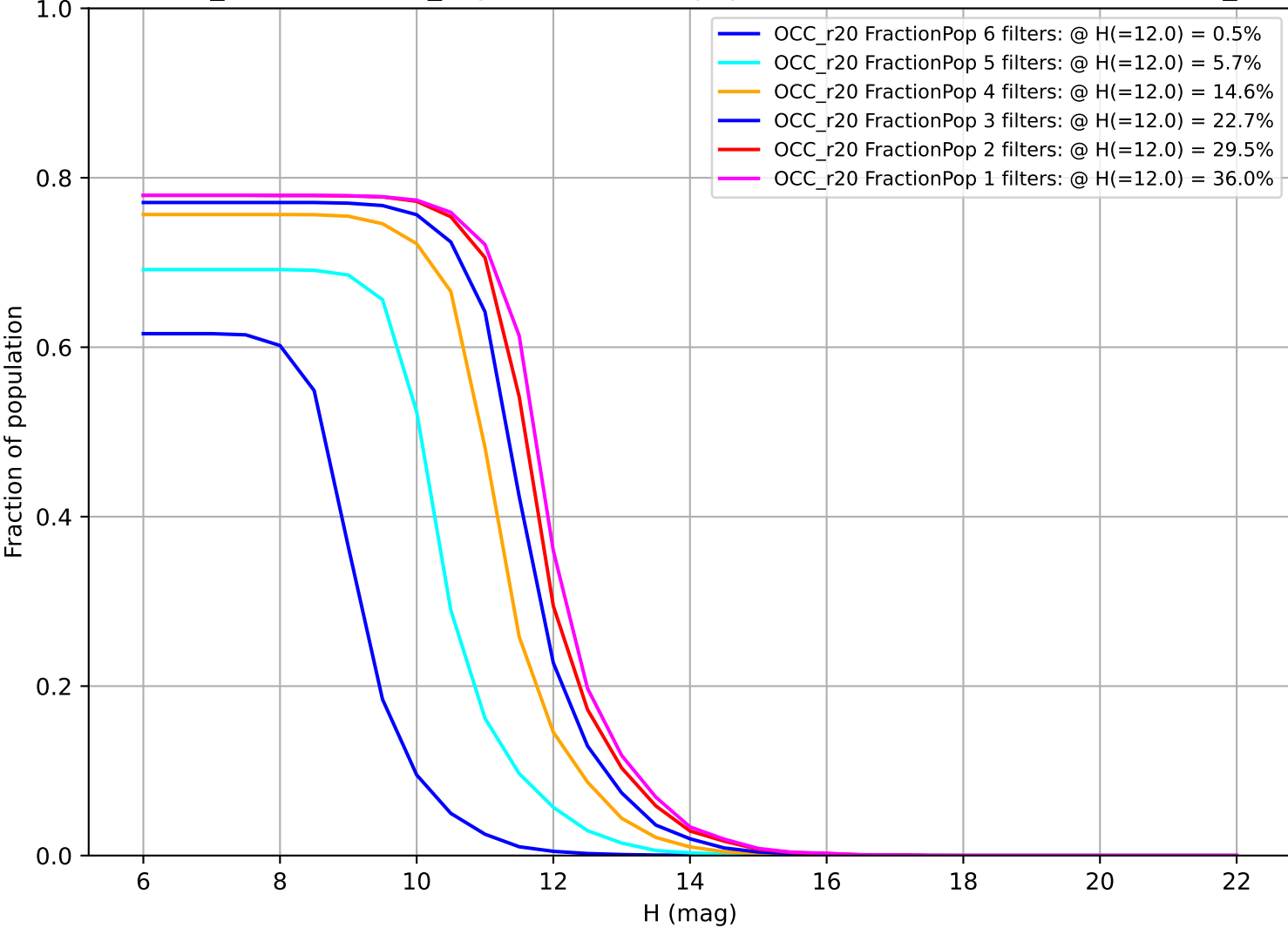
weather_cloudso35v3.5_10yrs: Fraction of population with colors in X filters OCC_r20
