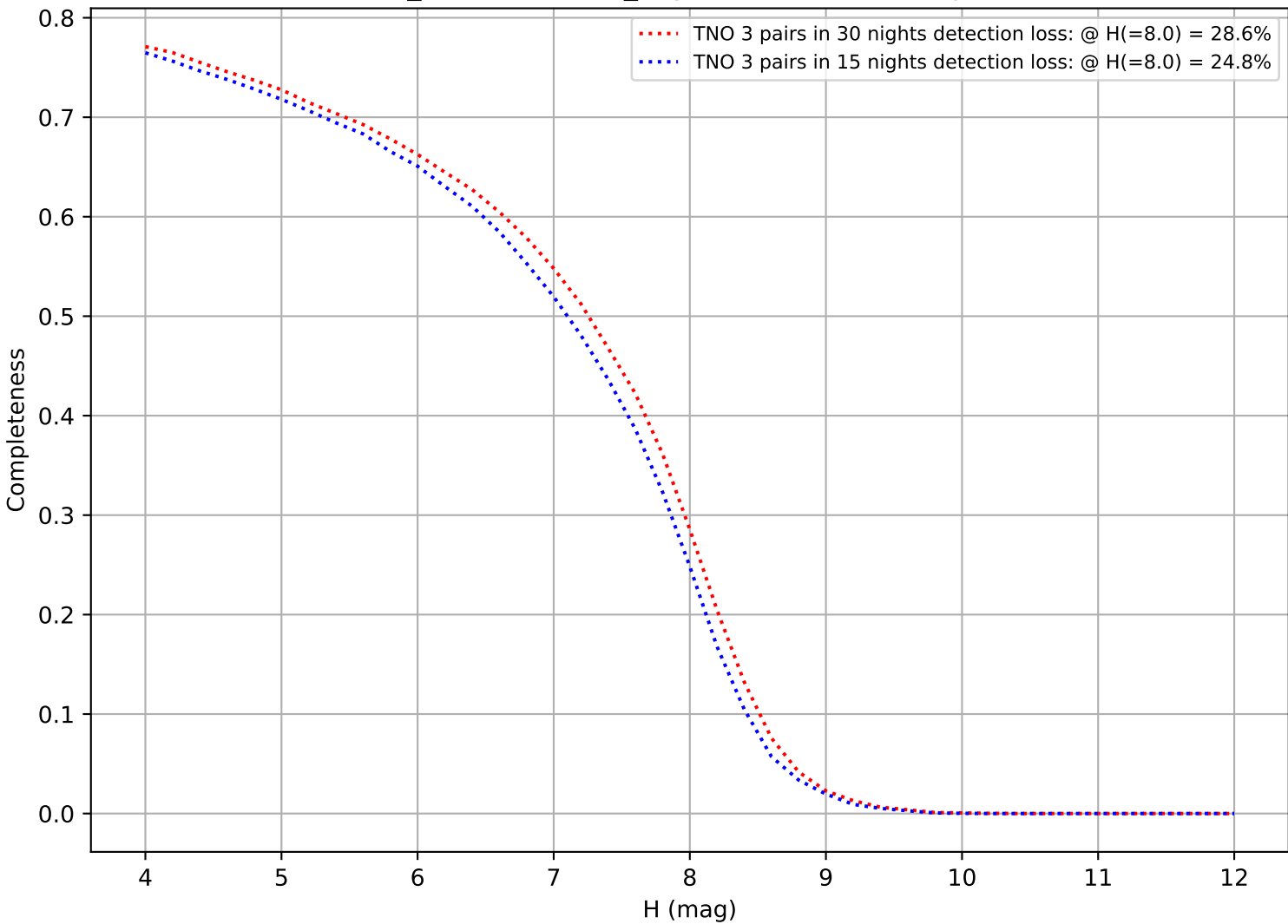
weather_cloudso35v3.5_10yrs: DifferentialCompleteness
