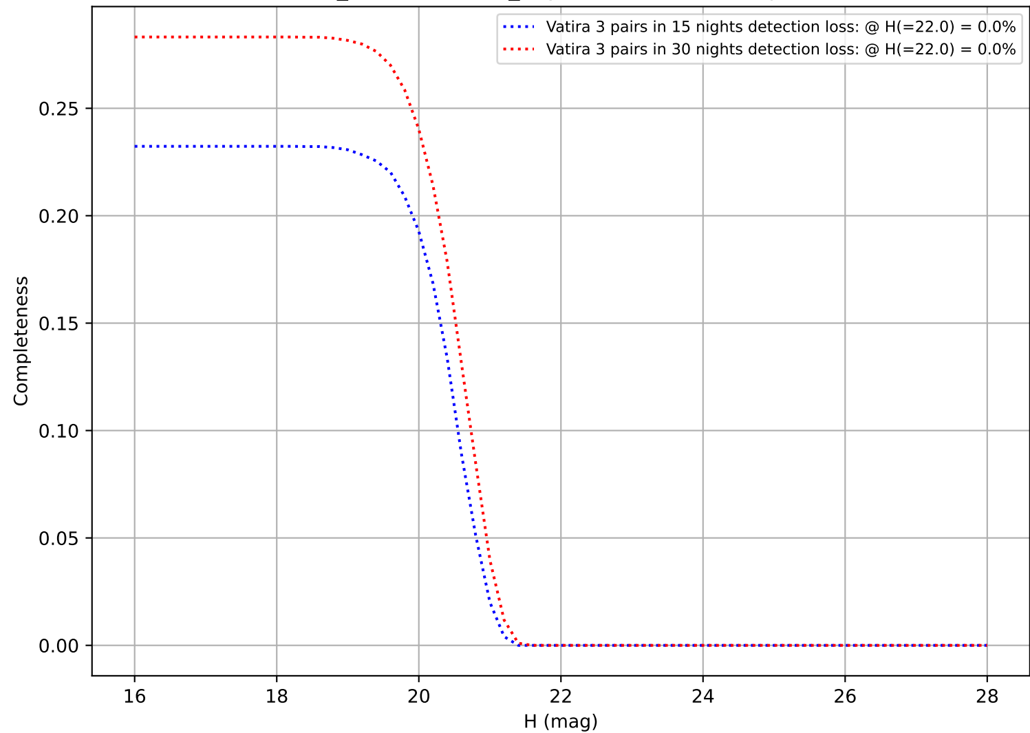
weather_cloudso35v3.5_10yrs: DifferentialCompleteness
