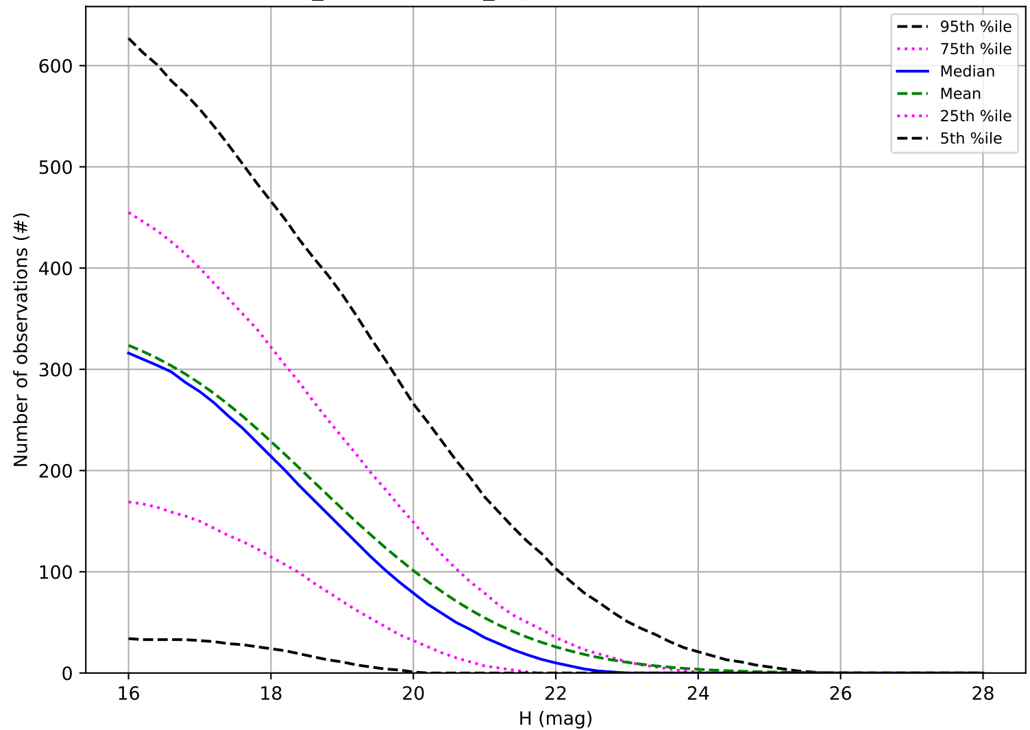
weather_cloudso35v3.5_10yrs: Number of observations NEO
