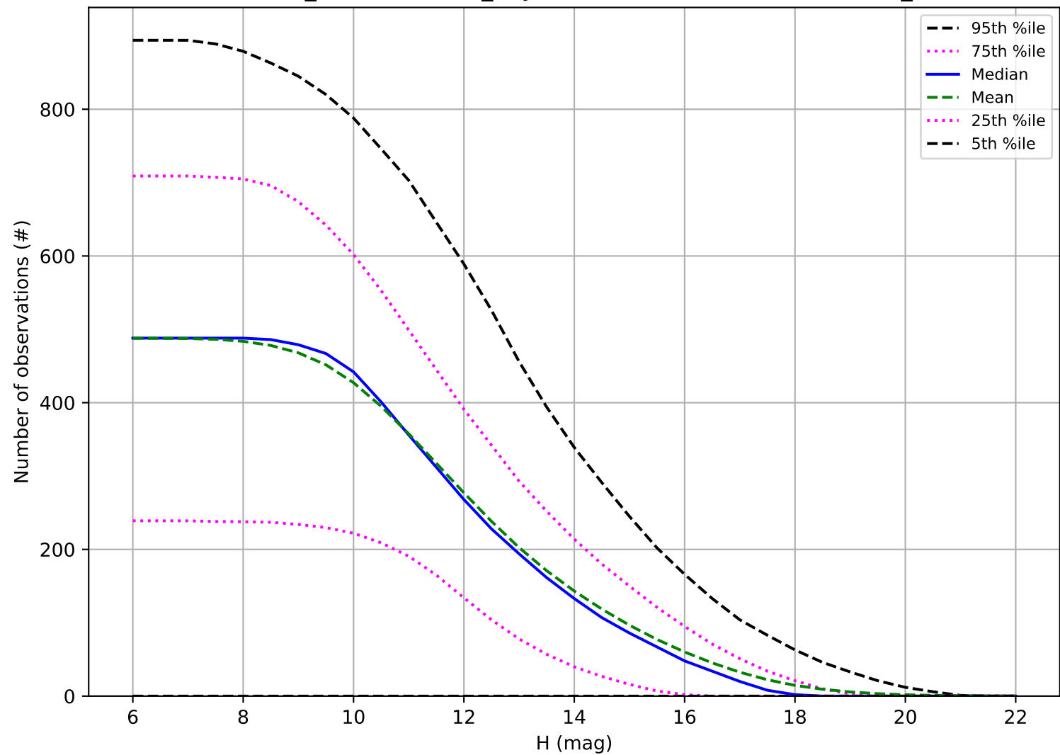
weather_cloudso35v3.5_10yrs: Number of observations OCC_r5
