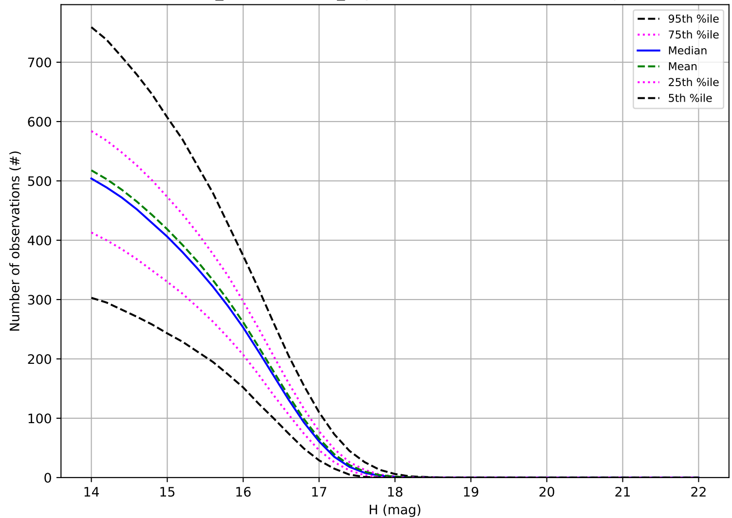
weather_cloudso35v3.5_10yrs: Number of observations Trojan
