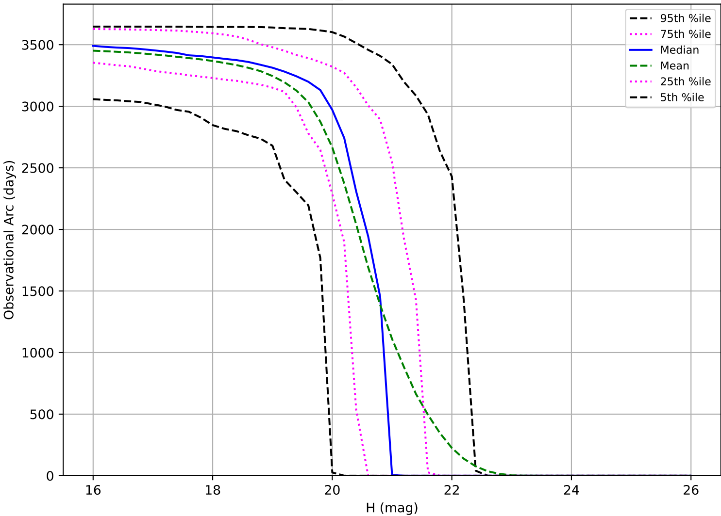
weather_cloudso35v3.5_10yrs: Observational Arc Length MBA
