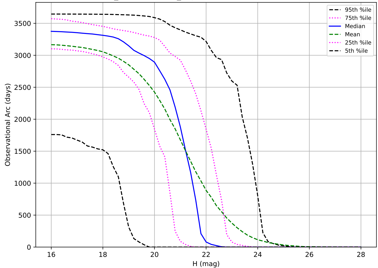
weather_cloudso35v3.5_10yrs: Observational Arc Length NEO
