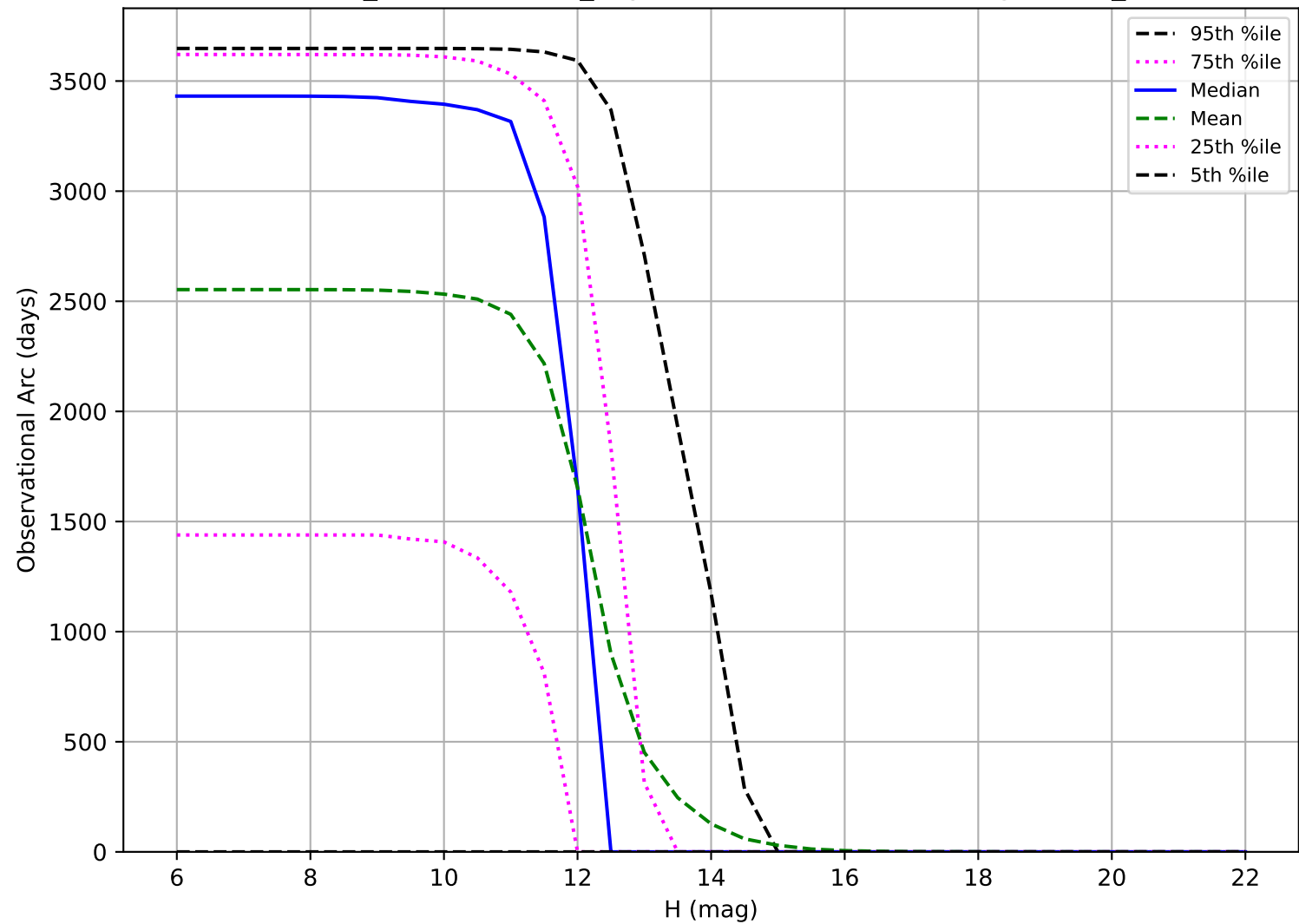
weather_cloudso35v3.5_10yrs: Observational Arc Length OCC_r20
