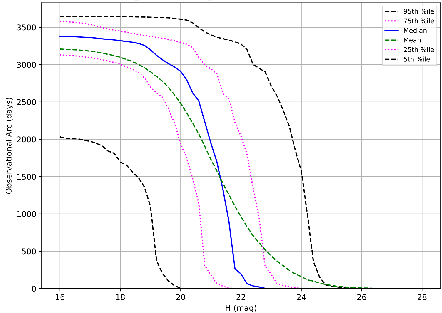
weather_cloudso35v3.5_10yrs: Observational Arc Length PHA
