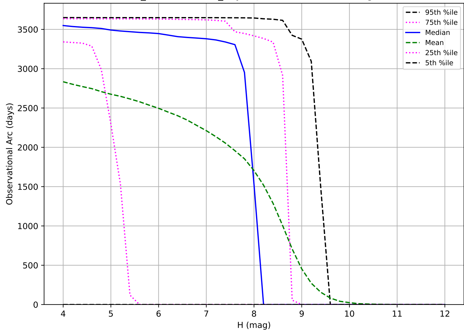
weather_cloudso35v3.5_10yrs: Observational Arc Length TNO
