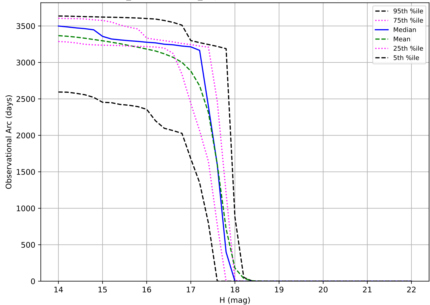
weather_cloudso35v3.5_10yrs: Observational Arc Length Trojan
