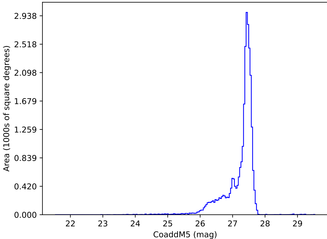
weather_cloudso36v3.5_10yrs : CoaddM5
