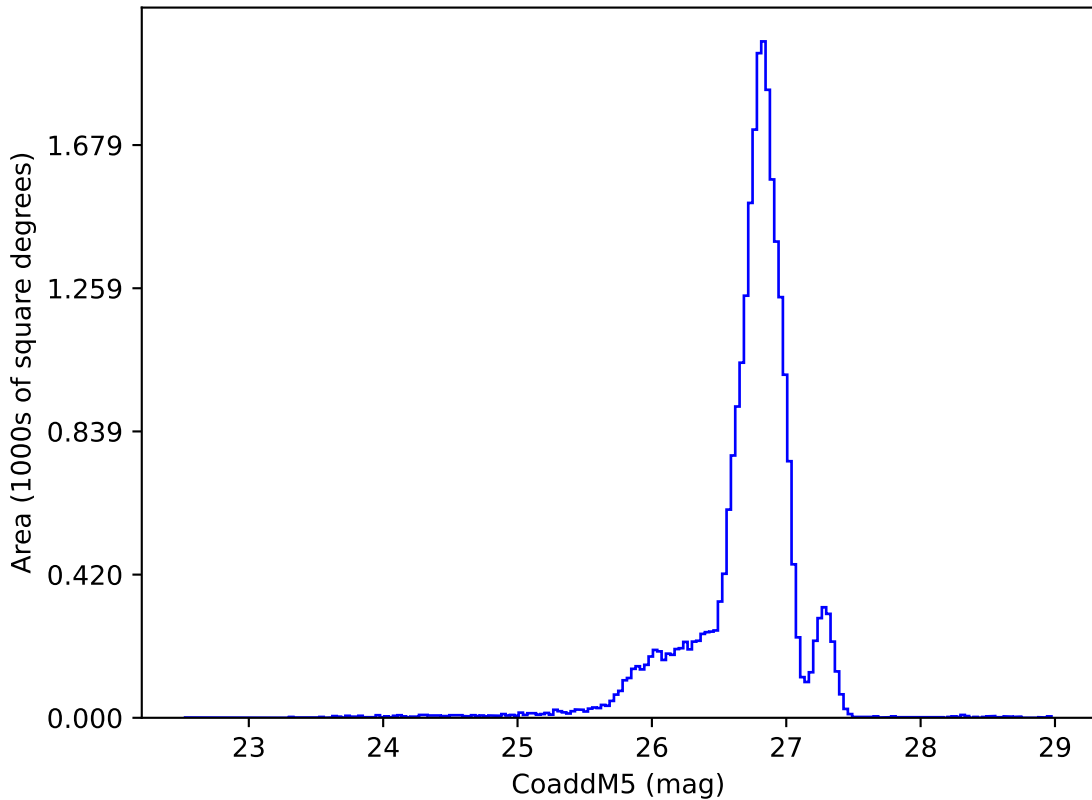
weather_cloudso36v3.5_10yrs g: CoaddM5
