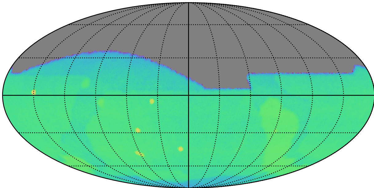
weather_cloudso36v3.5_10yrs g: CoaddM5
