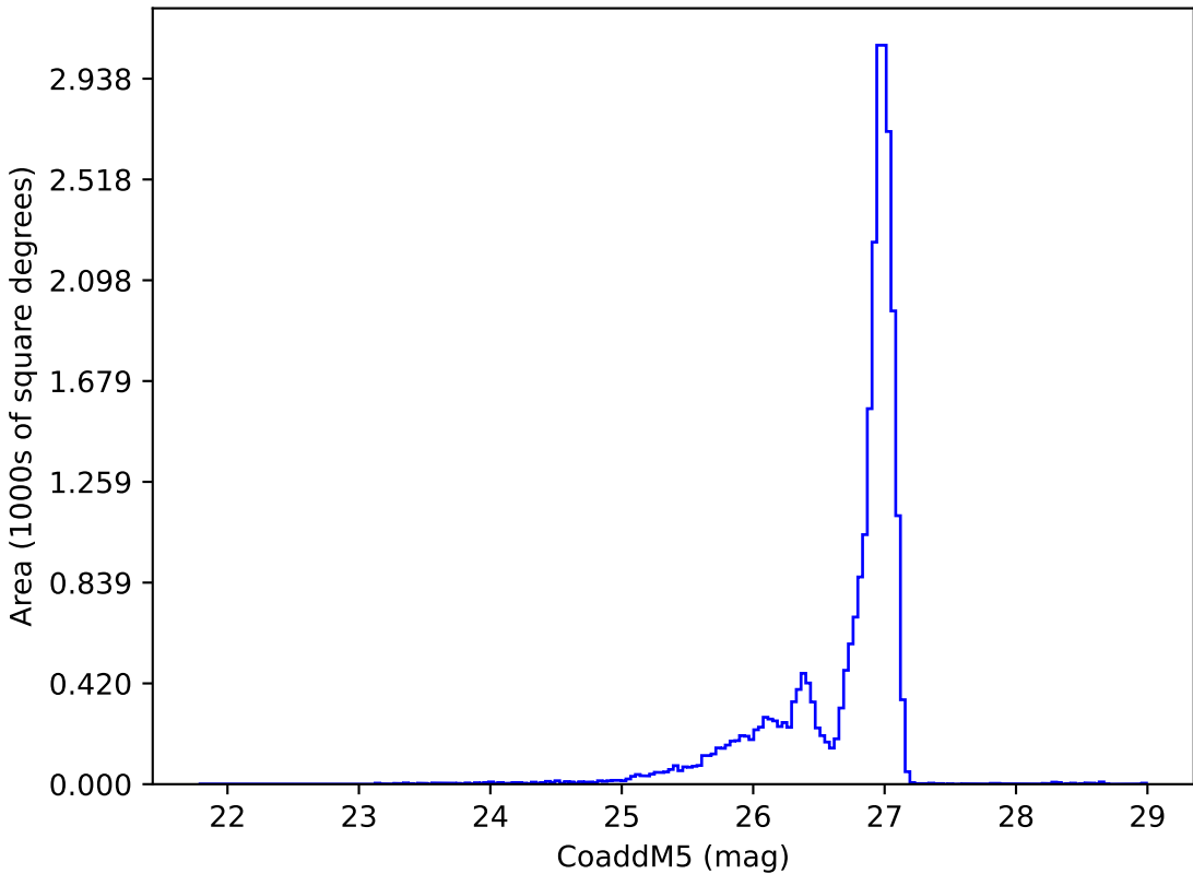
weather_cloudso36v3.5_10yrs r: CoaddM5
