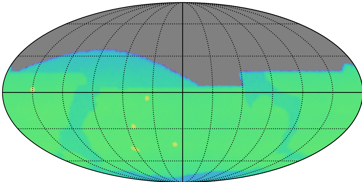
weather_cloudso36v3.5_10yrs r: CoaddM5
