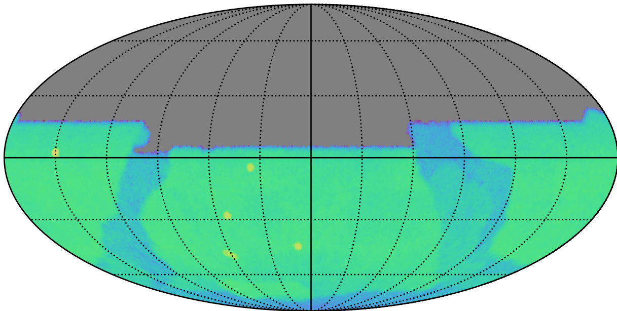
weather_cloudso36v3.5_10yrs u: CoaddM5
