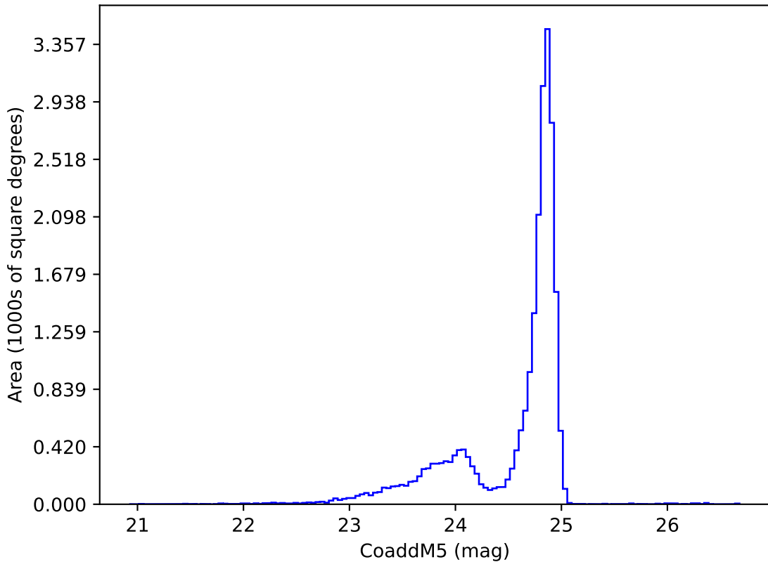
weather_cloudso36v3.5_10yrs y: CoaddM5
