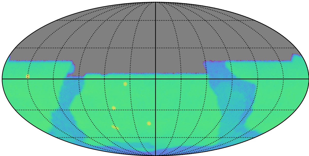
weather_cloudso36v3.5_10yrs y: CoaddM5
