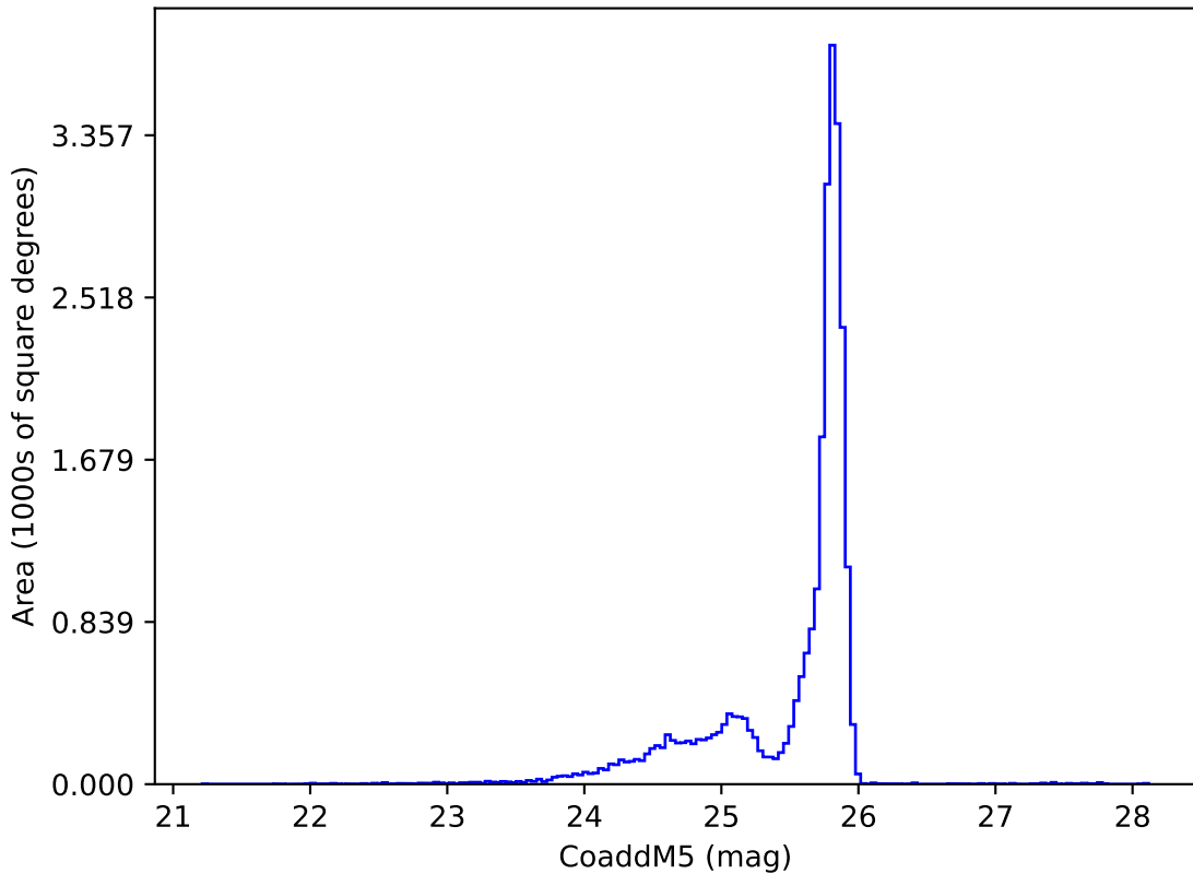
weather_cloudso36v3.5_10yrs z: CoaddM5
