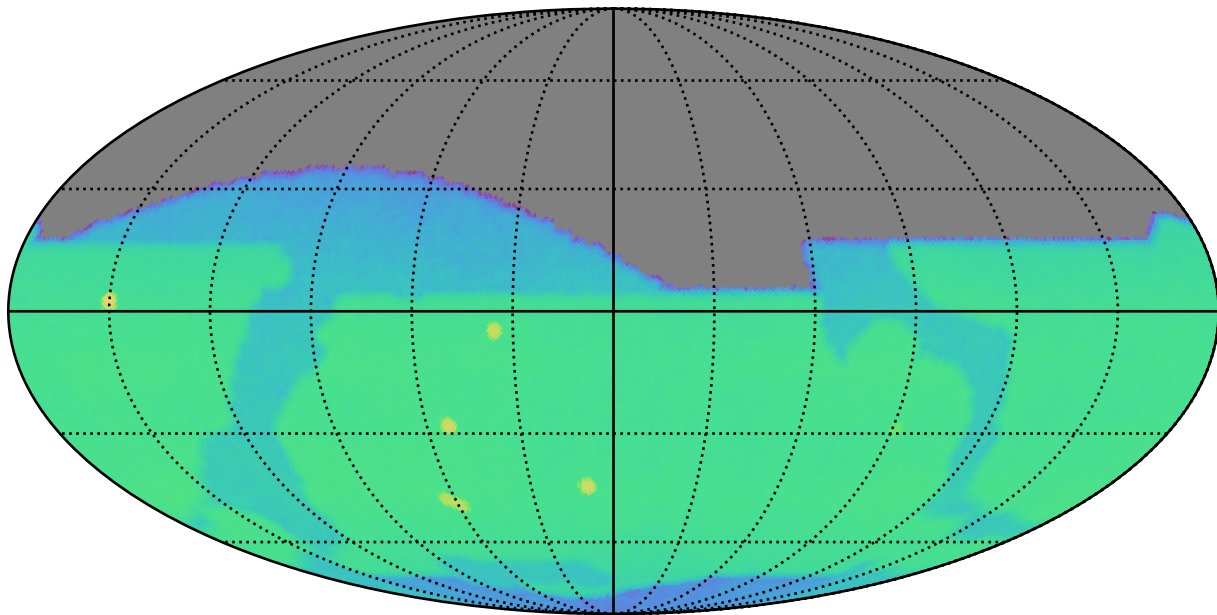
weather_cloudso36v3.5_10yrs z: CoaddM5
