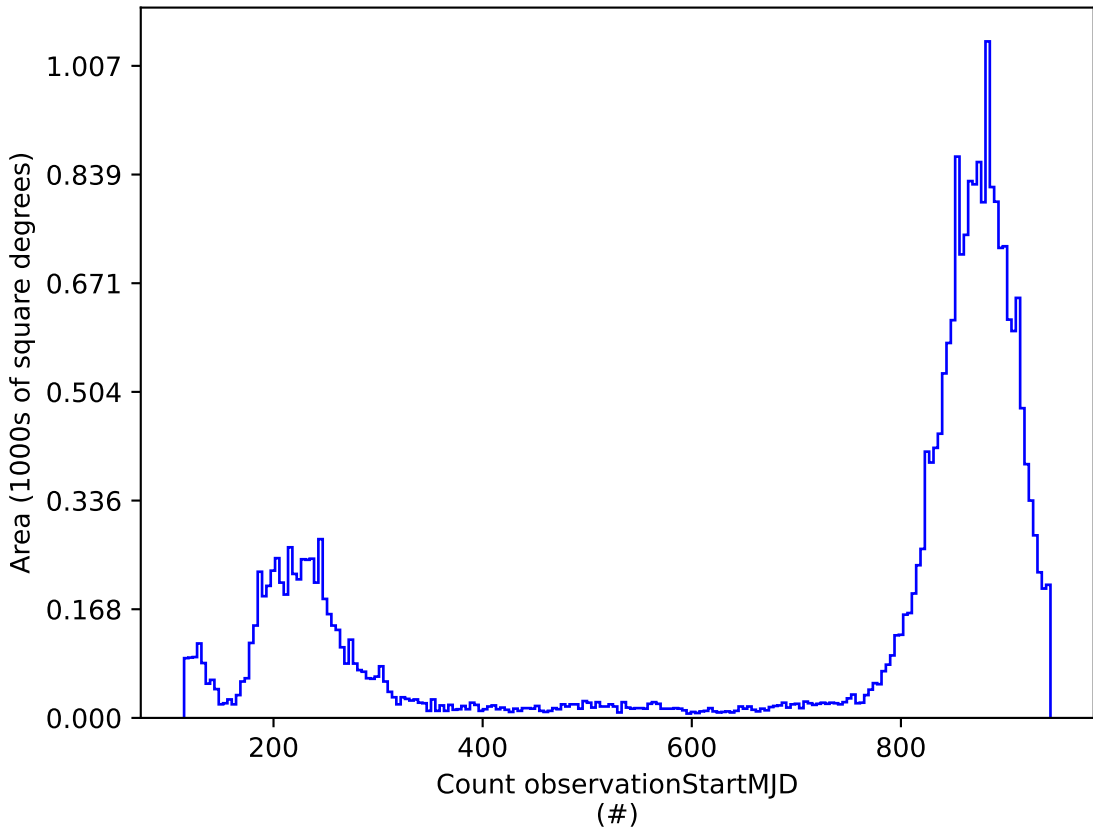
weather_cloudso36v3.5_10yrs : Count observationStartMJD
