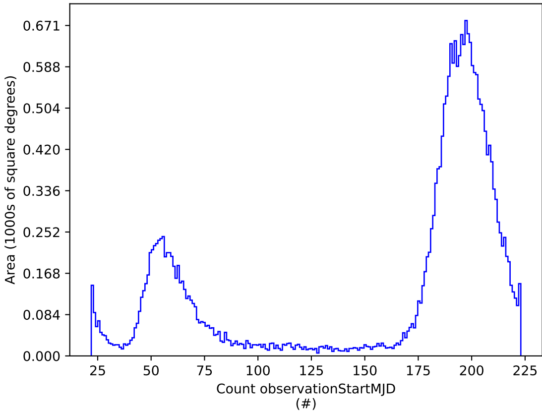
weather_cloudso36v3.5_10yrs i: Count observationStartMJD
