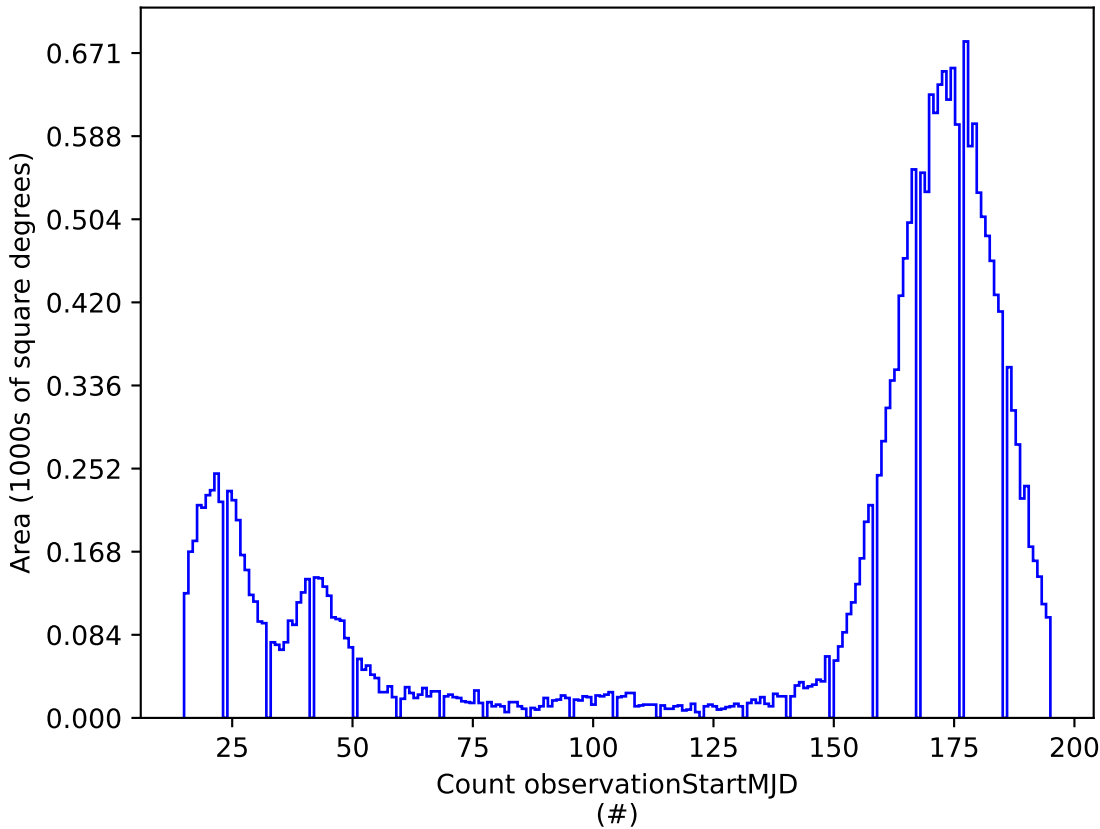
weather_cloudso36v3.5_10yrs y: Count observationStartMJD
