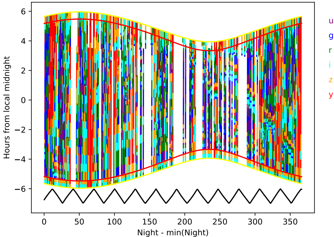
weather_cloudso36v3.5_10yrs year 0-1: Hourglass
