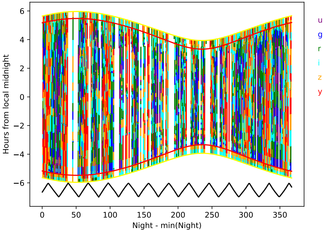
weather_cloudso36v3.5_10yrs year 3-4: Hourglass
