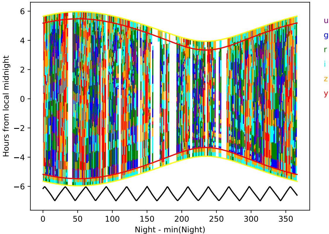
weather_cloudso36v3.5_10yrs year 9-10: Hourglass
