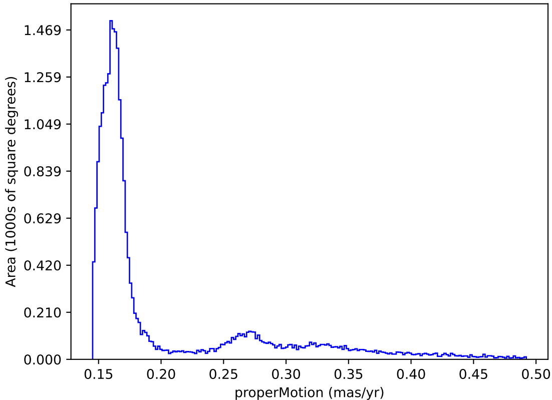
weather_cloudso36v3.5_10yrs : properMotion
