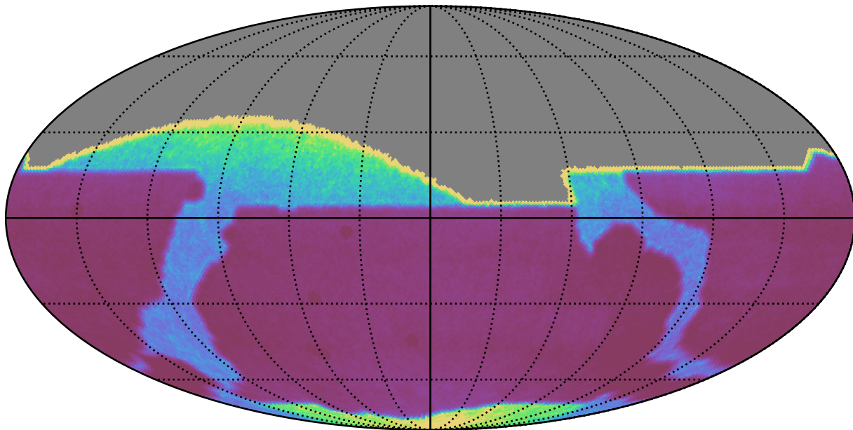
weather_cloudso36v3.5_10yrs : properMotion
