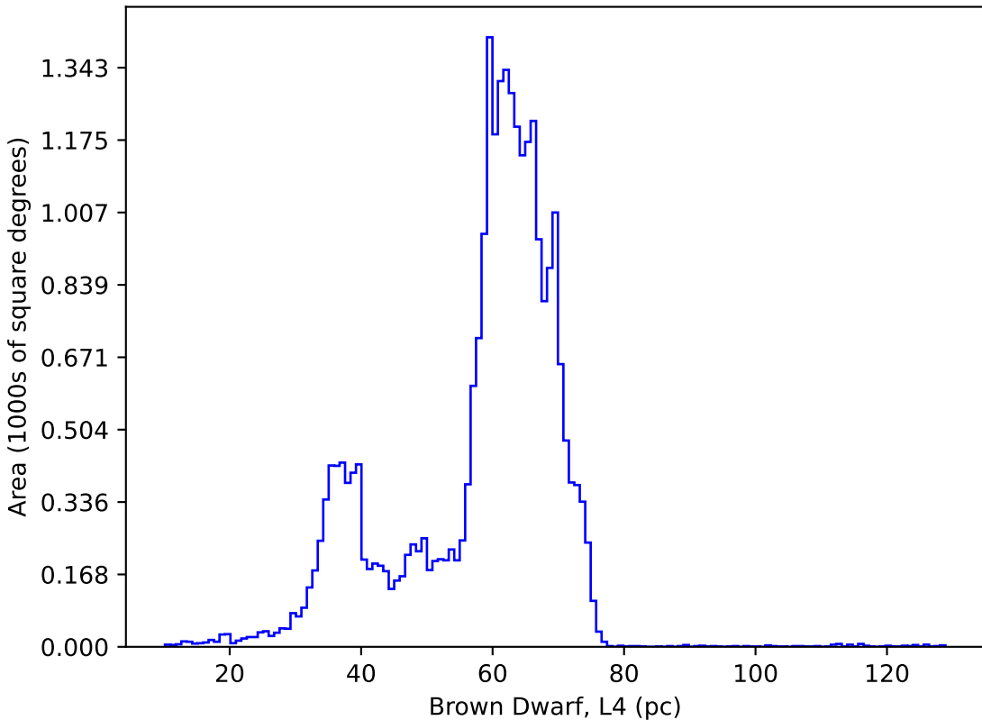
weather_cloudso36v3.5_10yrs : Brown Dwarf, L4
