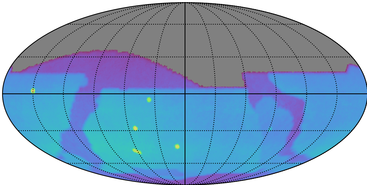
weather_cloudso36v3.5_10yrs : Brown Dwarf, L4
