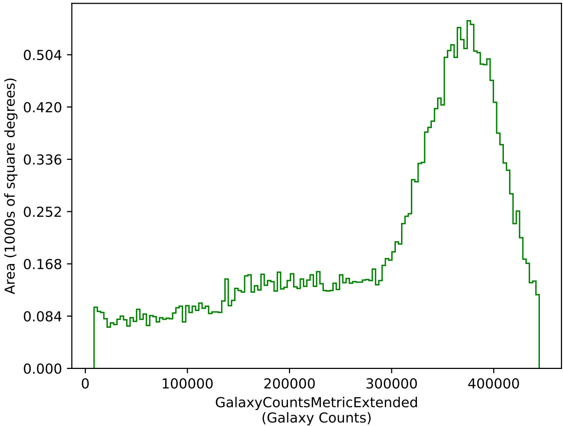
weather_cloudso36v3.5_10yrs g: GalaxyCountsMetricExtended
