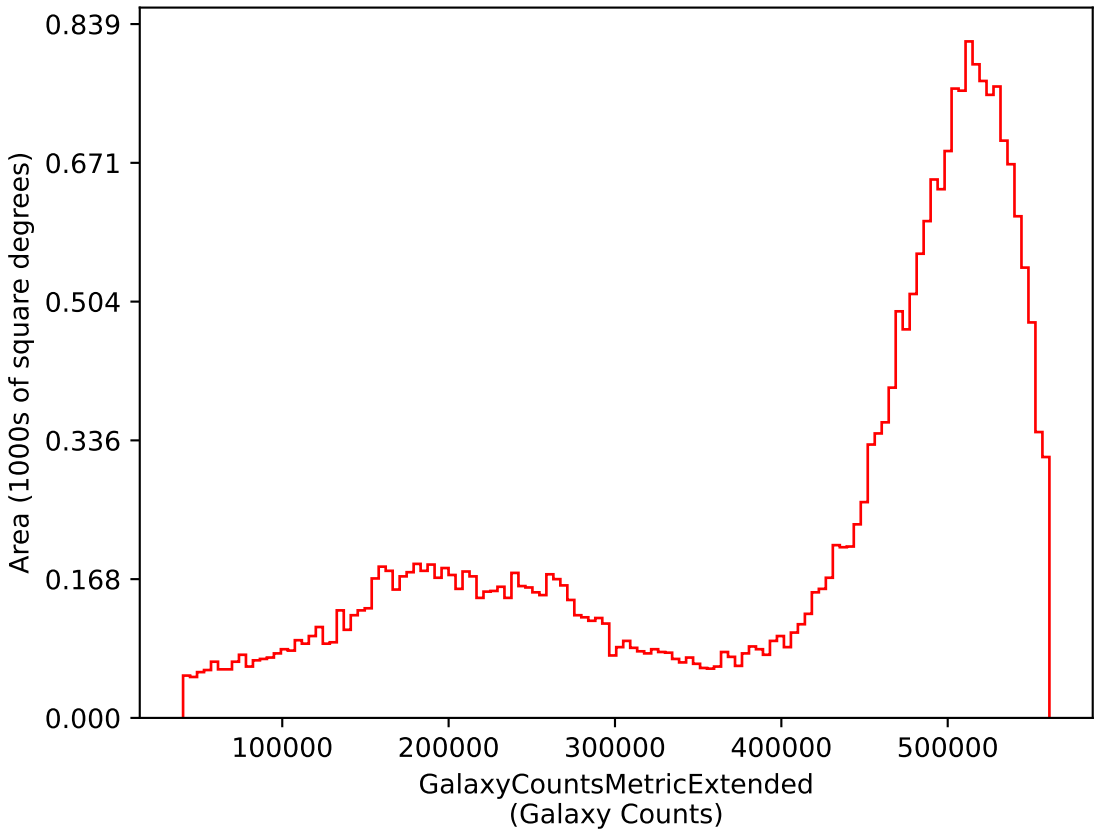
weather_cloudso36v3.5_10yrs i: GalaxyCountsMetricExtended
